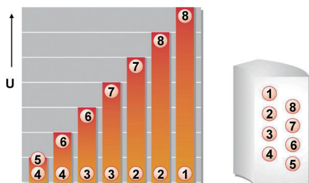
Round-wire winding
