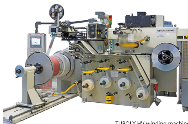
TUBOLY HV winding machine
