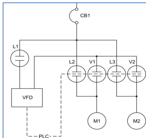
Figure 11: Optimized multi-motor synchronous transfer
