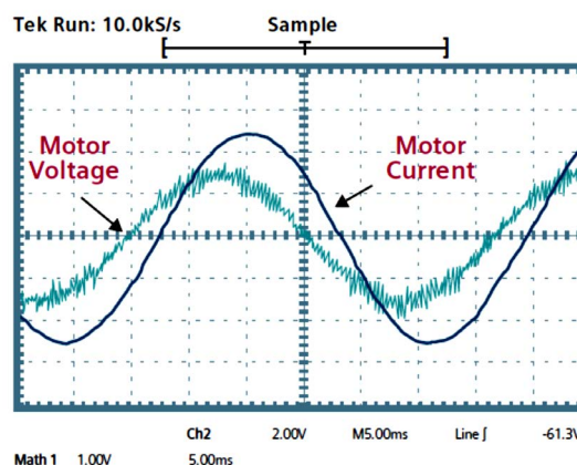
Figure 14: Output waveform
