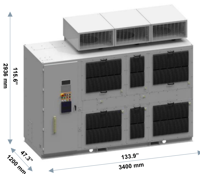
Frame 3B, 12/15 cell, 1500 to 3500 HP, 200/260 A
