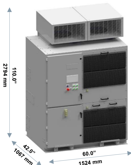
Frame 2A, 9 cell, 400 to 1100 HP, 100/140 A (and 40/70 A for drives manufactured in China)
