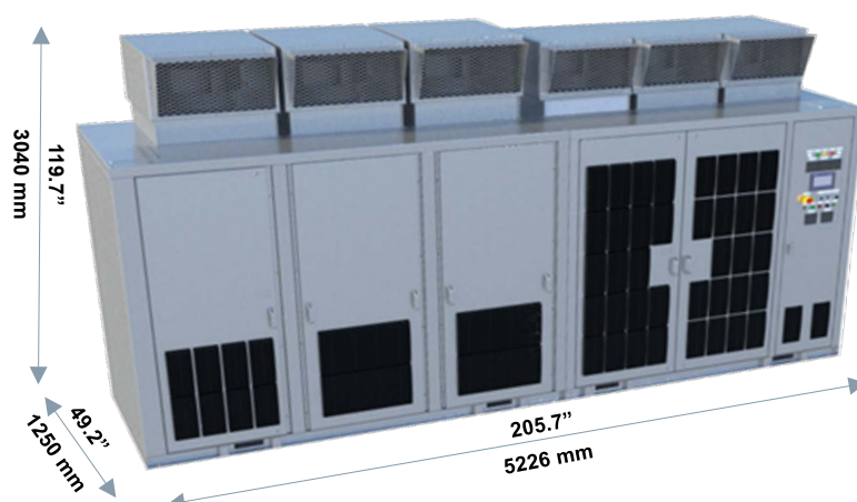
Frame 3D, 24 cell, 1750 to 5750 HP, 200/260 A 2)
