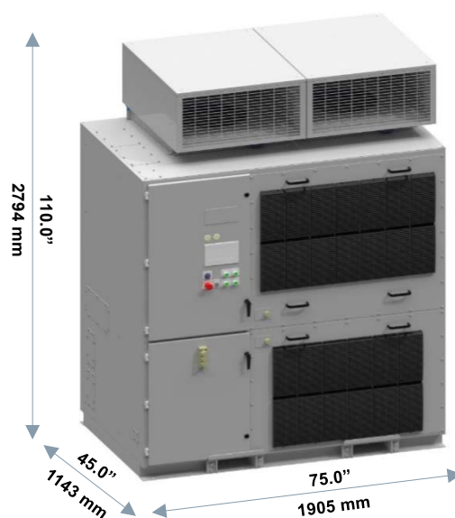
Frame 3A, 9 cell, 300 to 2000 HP, 200/260 A
