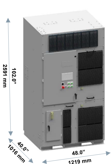
Frame 1A, 150 to 500 HP, 40/70 A (except for drives manufactured in China)
