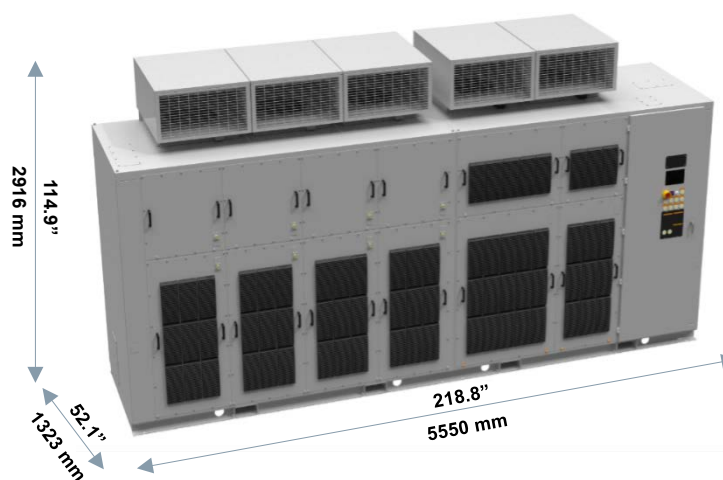
Frame 4B, 12/15 cell, 2500 to 5500 HP, 340/430 A
