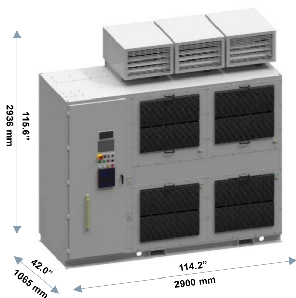
Frame 2B, 12/15 cell, 300 to 1750 HP, 40 to 140 A
