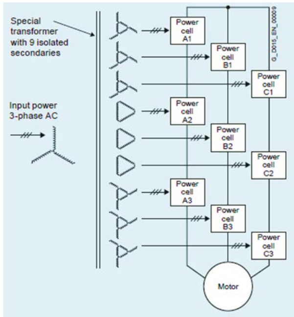
Figure 1: Topology of Perfect Harmony GH180 drive (3 cells per phase)
